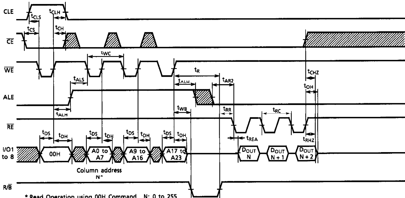
Read Cycle (1) Timing Diagram: Interrupted by CE
