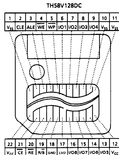
Figure 1. Pinout
