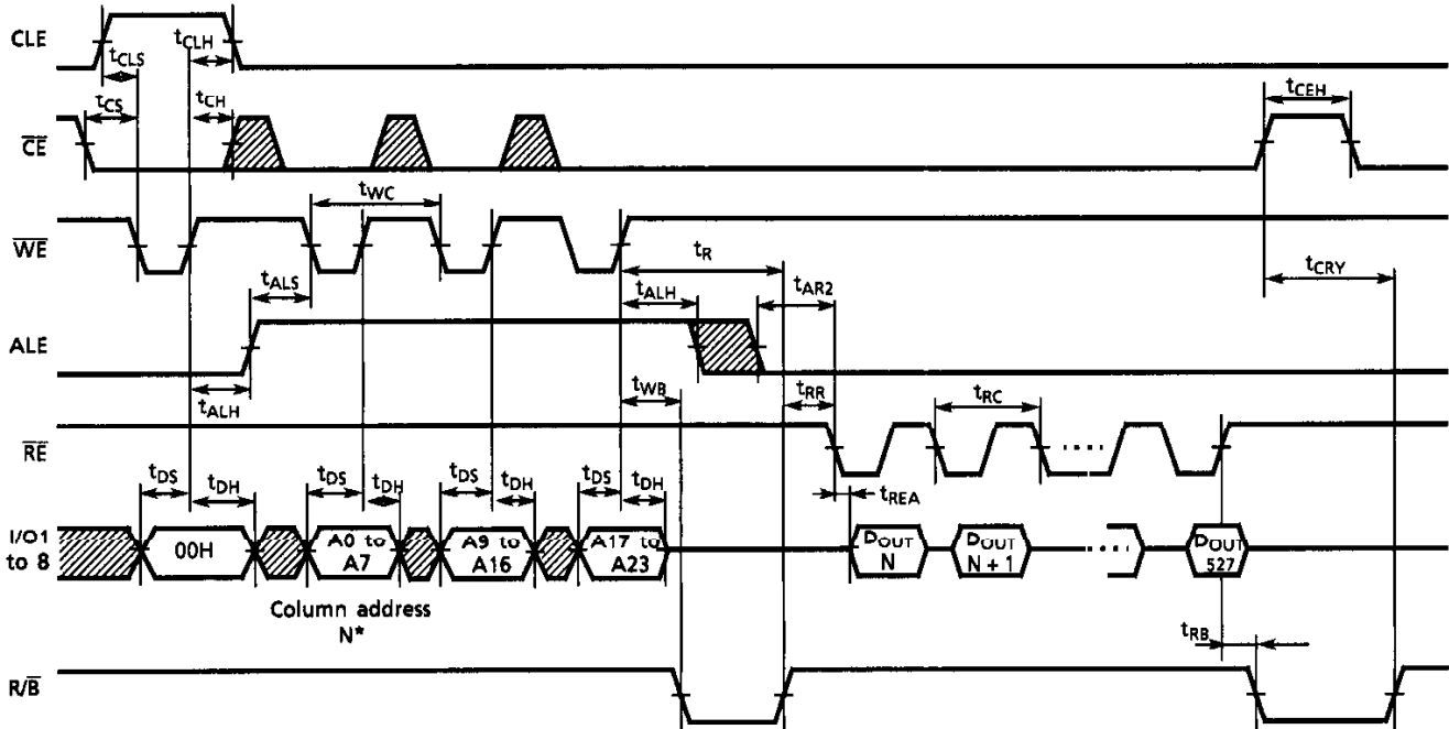
Read Cycle (1) Timing Diagram
