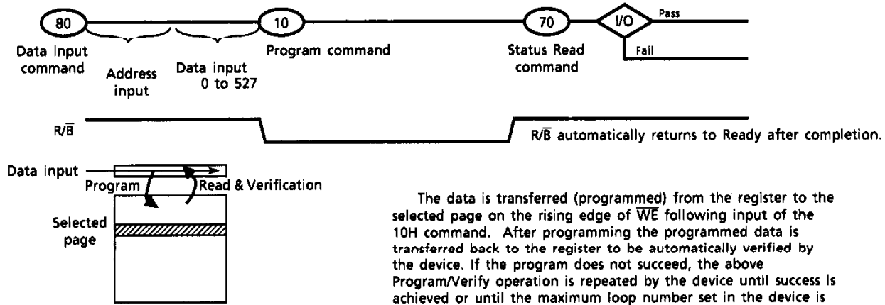
Figure 7. Auto Page Program operation
