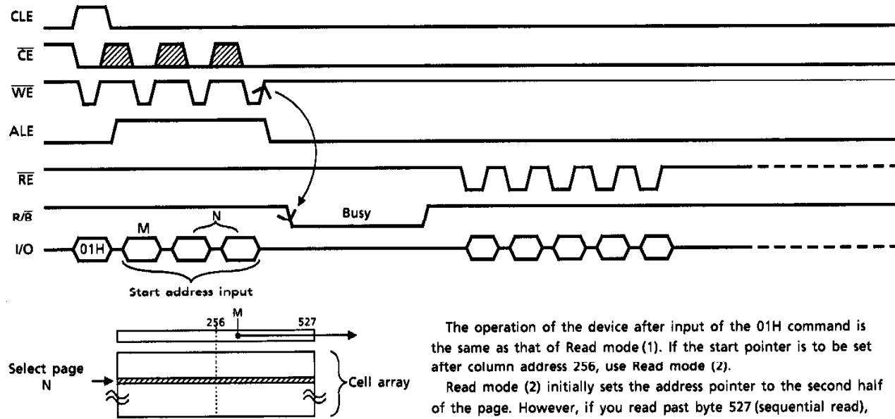
Figure 4. Read mode (2) operation
